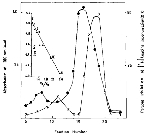
Fig.2. Chromatography of hpO_2I on Sephadex G-100. 6.2 mg protein enriched in hpO_2I activity by (NH_4)_2SO_4 -precipitation between 0–50% saturation were applied to G-100 column ( 1 \times 45 cm), equilibrated and eluted in TKMM buffer. 1 ml fractions were collected and 15 \mu l aliquots were assayed for hpO_2I activity in protein synthesis [5]. Control activity (0% inhibition) was 7500 cpm/20 \mu l reaction mixture. V_0 (void volume) = 8.8 ml. The inset shows the repetition of the experiment on a second G-100 column ( 1 \times 42 cm) calibrated with: (1) adenosine diphosphate ribosylated-elongation factor 2 (96 500) [7]; (2) creatine kinase (80 000); (3) bovine serum albumin (68 000); (4) ovalbumin (45 000); and (5) cytochrome c (12 500). V_e/V_0 ratios, where V_e = elution volume corresponding to the peak concentration of each (standard) protein and V_0 = void volume of the column (= 8.3 ml), were determined and plotted against log molecular weights. (I) corresponds to the hpO_2I activity eluting behind the void volume and (II) to the hpO_2I -activity eluting behind the main A_{280} peak. V_e used for hpO_2I (I) (= 8.5 \pm 0.5 ml) and V_e for hpO_2I (II) (= 17.4 \pm 1.5 ml) are means from four determinations. A third inhibitory activity of small molecular weight eluting with V_e = 29 \pm 2 ml has not been investigated further and is not shown in the diagram.
